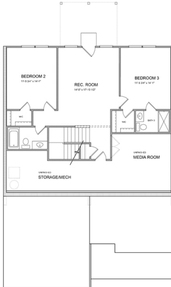
Terrace Level
