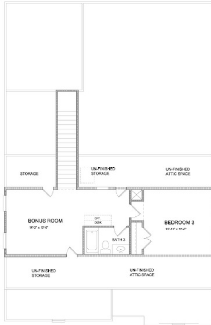
SECOND FLOOR
