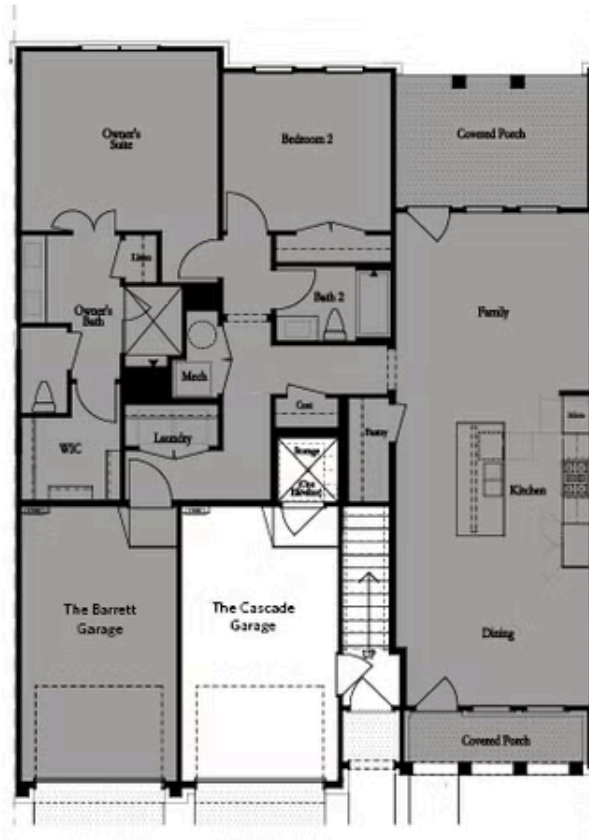
Garage Level
