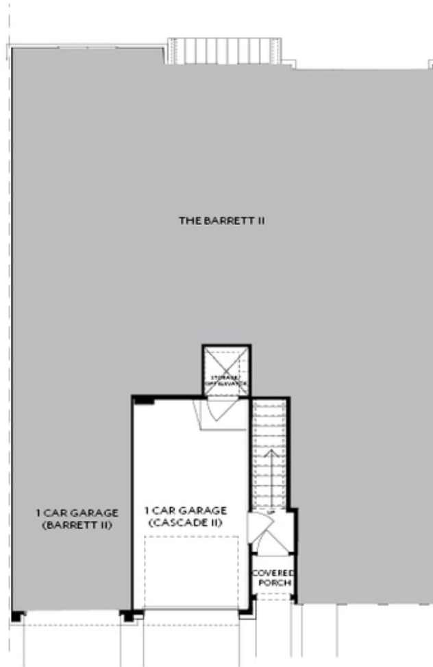
GARAGE LEVEL
