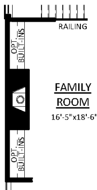
FIREPLACE WALL OPT. 5
